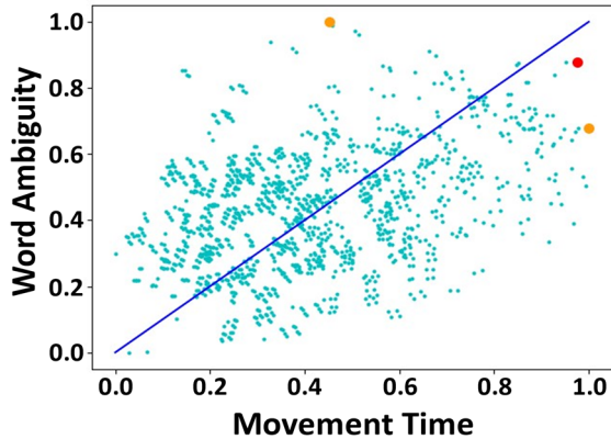
Figure 10. Candidate layouts shown by movement time score and word ambiguity score (orange dots: optimal layouts for single metric; red dot: final layout of BiTipText).
